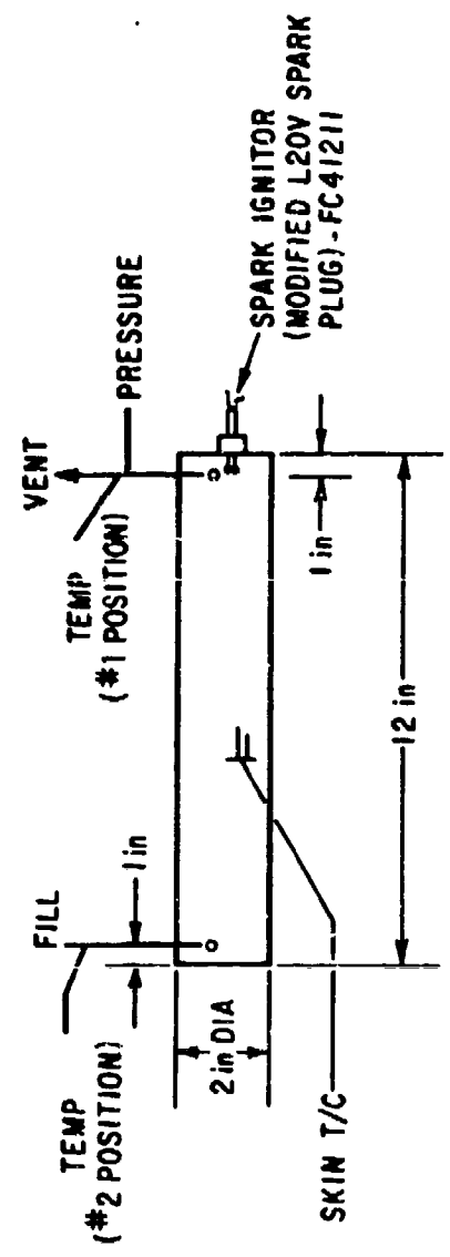
Figure 16. Ignition Apparatus
